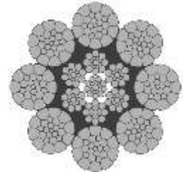
PYTHON Super 8-C
