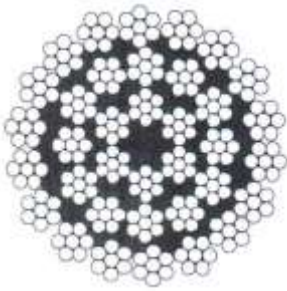
36x7 HERCULES standard
