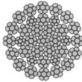
35x7 PYTHON compact
